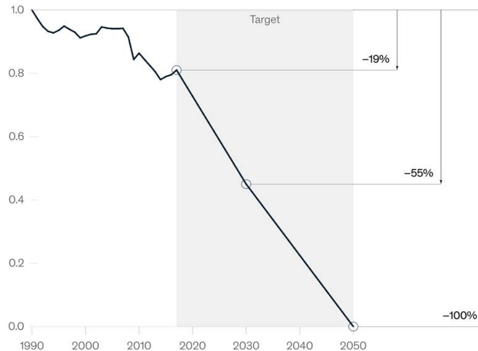
EU emissions development, index (1990 = 1.0) 1
